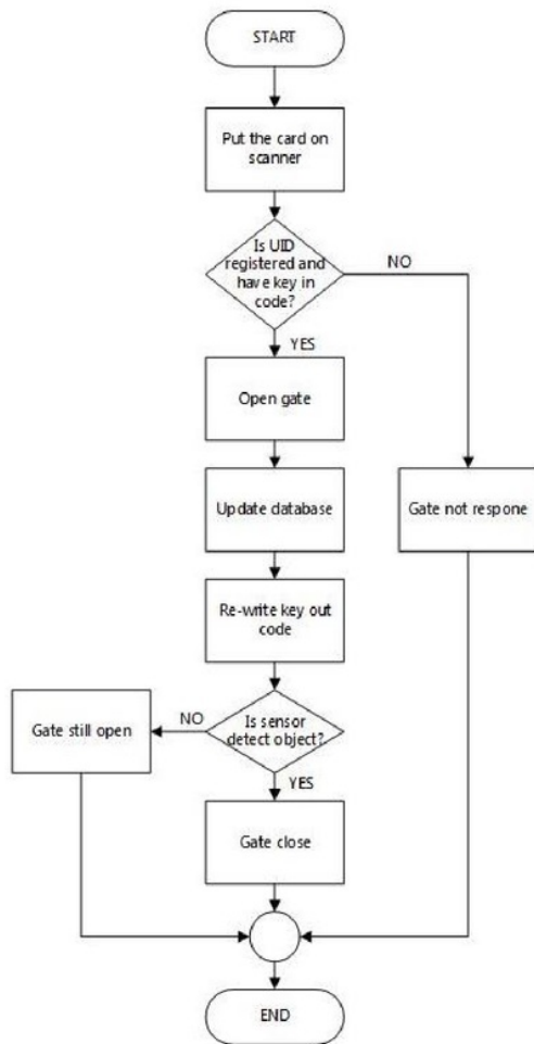
Fig. 3 Flowchart System Smart Gate Access Control
